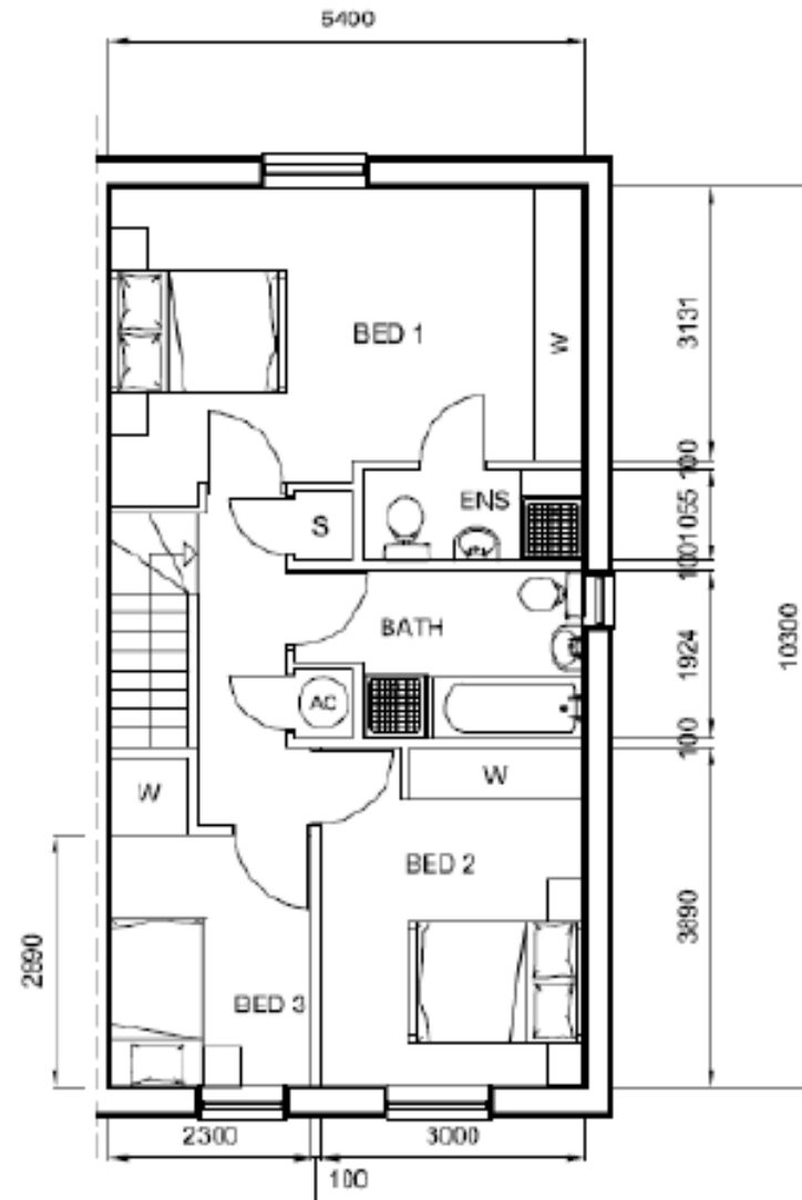
H1 02 3 BED HOUSE FIRST FLOOR PLAN GROSS INTERNAL FLOOR AREA 599 SQ FT
