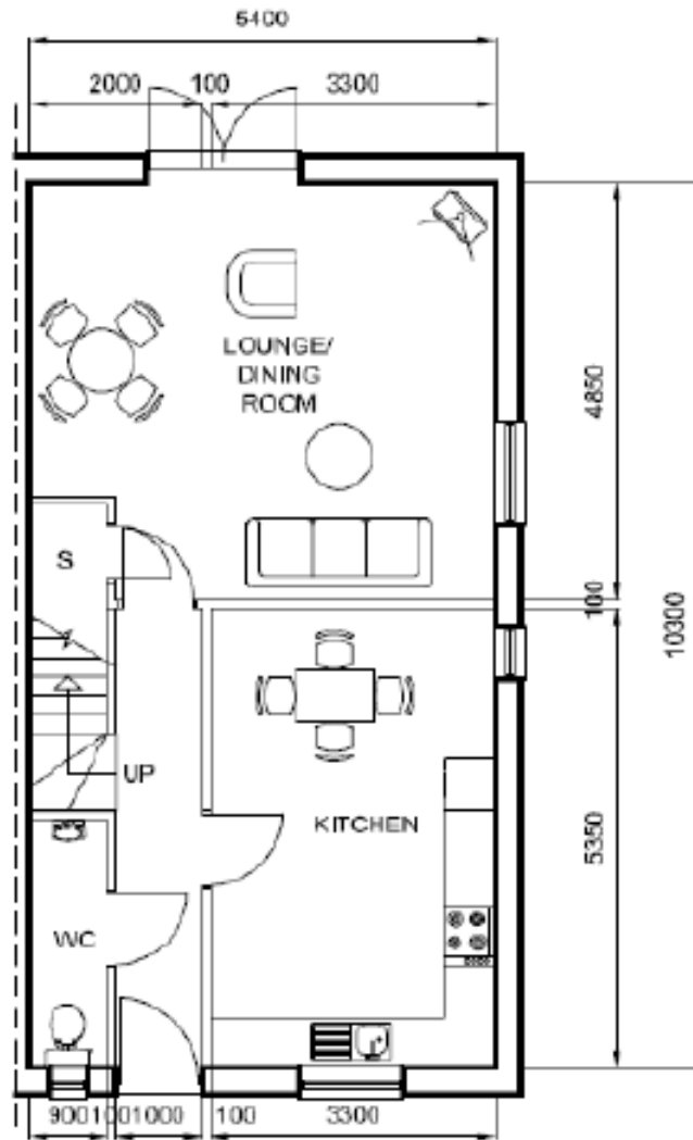
H1 01 3 BED HOUSE GROUND FLOOR PLAN GROSS INTERNAL FLOOR AREA 599 SQ FT
